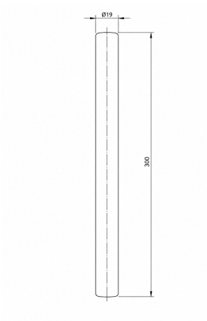
TECHNICAL DIMENSIONS
