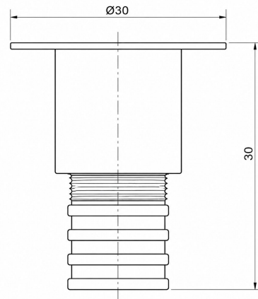
TECHNICAL DIMENSIONS
