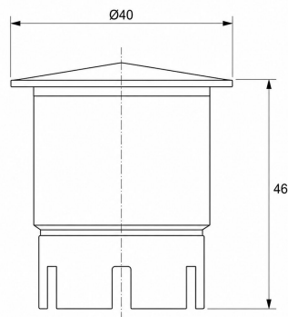
TECHNICAL DIMENSIONS
