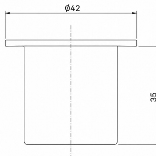
TECHNICAL DIMENSIONS
