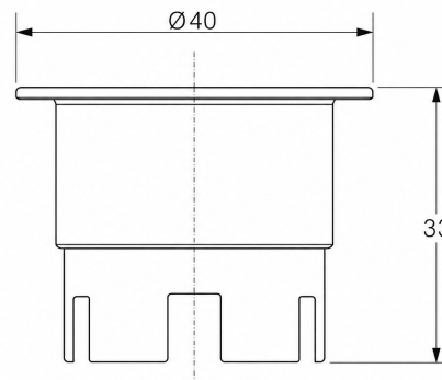
TECHNICAL DIMENSIONS
