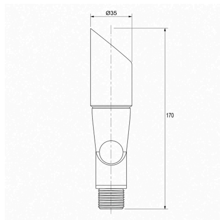
TECHNICAL DIMENSIONS
