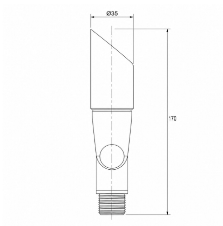
TECHNICAL DIMENSIONS
