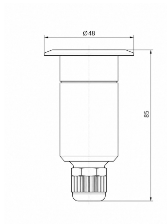
TECHNICAL DIMENSIONS
