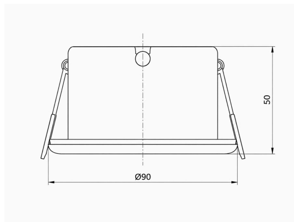
TECHNICAL DIMENSIONS
