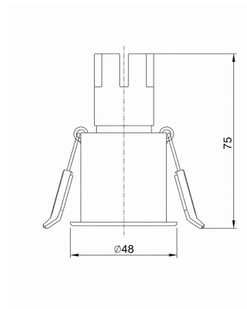
TECHNICAL DIMENSIONS
