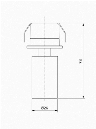
TECHNICAL DIMENSIONS
